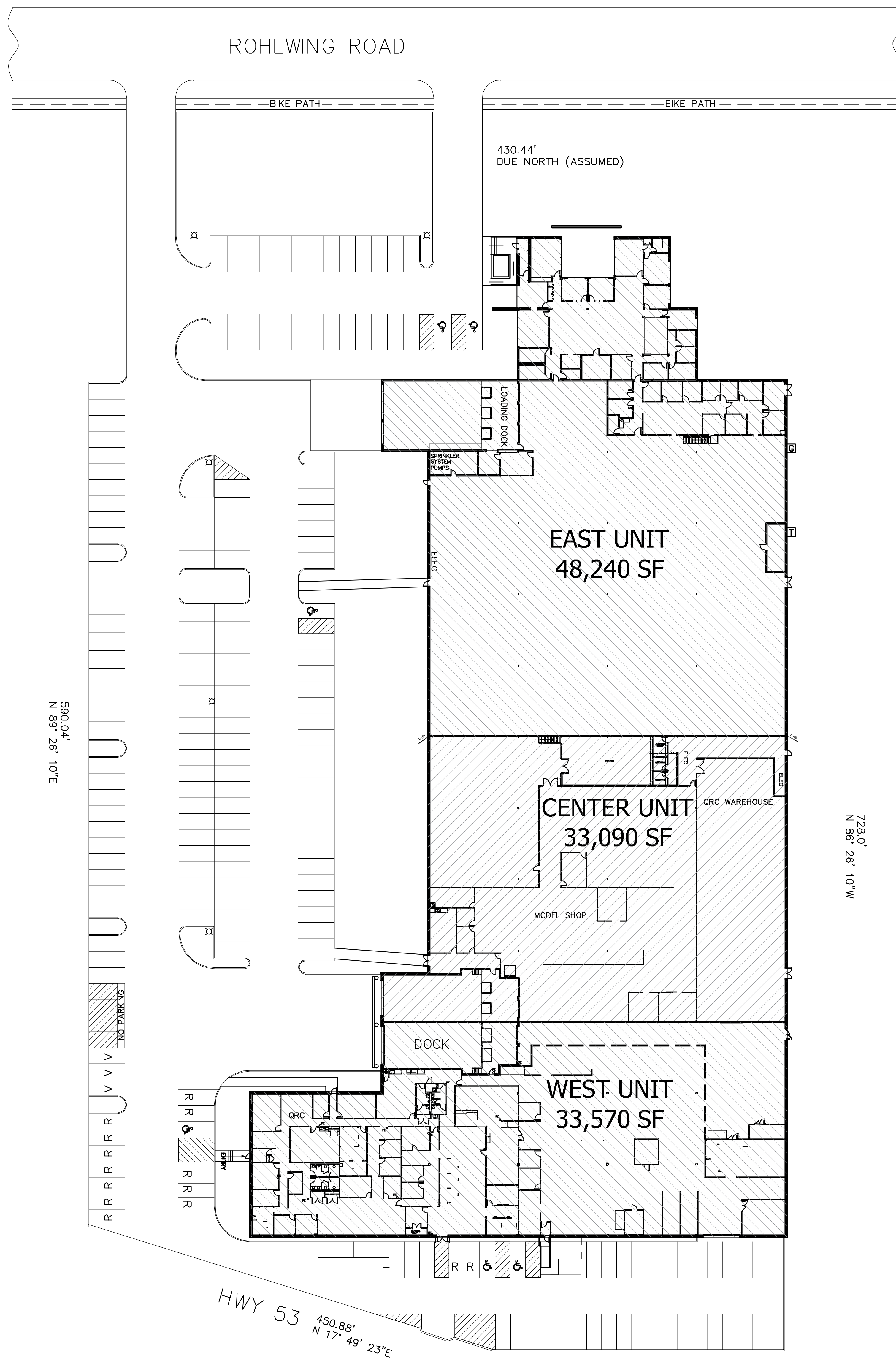
1 OVERALL PLAN SCALE: 1/32" = 1'-0"
